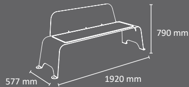
Bench with entire backrest
